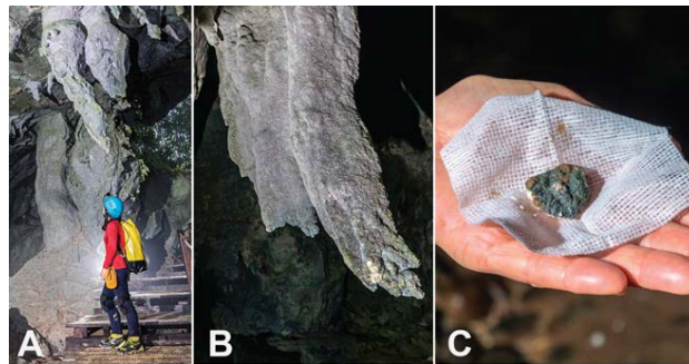
Figure 5. Curved stalactites. A) The entrance to Stonehorse Cave; B) Phyto-gen in Racer Cave; C) Fragment collected from the speleothem in B, with the obvious green cyanobacterial biofilm (Photos by Chris Howes).
