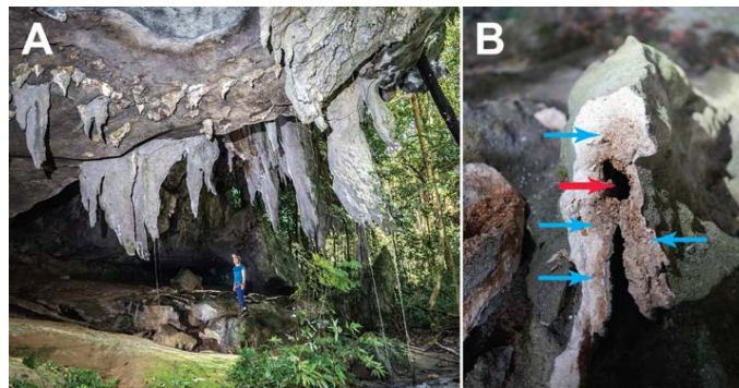
Figure 6. A) Roots are often associated with the curved stalactites, and seen emerging from the bottom. B) A broken stalactite reveals the presence of a central canal (red arrow), surrounded by a layer of what appears to be brown organic material (blue arrows). Photo A by Chris Howes.
