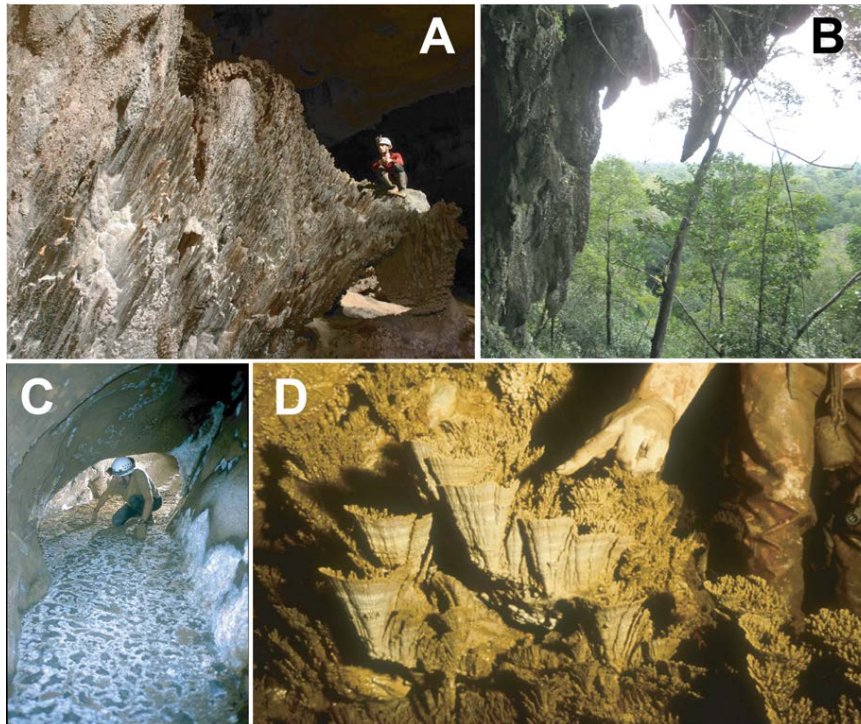
Figure 1. Potential biogenic formations within the caves of Gunung Mulu National Park. A) The long spikes of phytokarst can be found in entrances throughout the park. These pinnacles appear to be caused by photosynthetic bacteria. B) At the entrance of many caves are curved stalactites that appear to curve toward sunlight. C) White encrustations may indicate the presence of saltpeter, \text{Ca}(\text{NO}_3)_2 , which may be biogenic in origin. D) There is no clear mechanism of formation of the fluted deposits seen in the cave.
