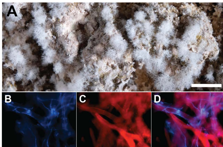
Figure 10. Gross and microscopic examination of fluffy moonmilk. A) Gross appearance of moonmilk with the fluffy tufts of material that are not normally associated with this formation (scale bar = 1 cm). B - D) Fluorescence microscopy of a tuft isolated from A . B is stained with the blue/white fungal-specific dye calcofluor; C is the autofluorescence of the same material - such autofluorescence is characteristic of calcite. D) Composite image of B and C , showing how the fungal material wraps around the calcite crystals.
