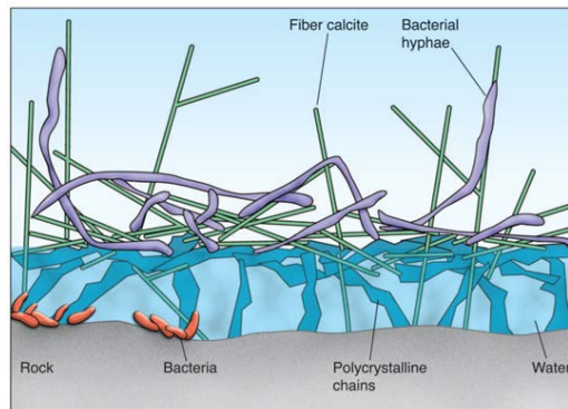
Figure 8. Model of moonmilk formation [from Barton and Jurado, 2007 (32)].
