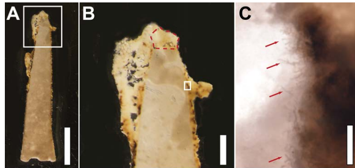
Figure 3. Thin-sections through phytokarst. A) Thin-section of a piece of phytokarst from Clearwater Cave (scale bar = 5 mm); B) Close-up of area indicated by white square in A . The limestone host rock of the phytokarst pinnacle is obvious in the thin-section, including its flat surface. The original calcification is indicated by the dotted red line, with additional calcite build-up seen on either side, and the brown organic residue of cyanobacterial growth along both edges (scale bar = 1 mm); C) Close-up of cyanobacterial growth highlighted by the white box in B . The brown organic matter of the cyanobacterial biofilm is obvious (to the right), along with individual bacetrial filaments boring into the limestone (indicated by red arrows; scale bar = 10 \mu m).
