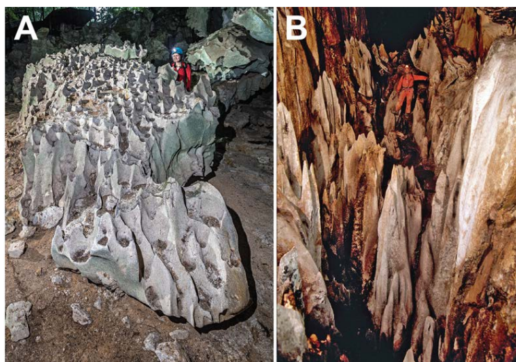
Figure 12. The impact of bird guano on rock surfaces within the Mulu caves. A) Initially, bird guano starts to accumulate on surfaces, creating pockets where the material begins to accumulate. Over time, these pockets allow much deeper deposits of guano to form, potentially speeding up nitric acid production, eventually creating very deep pockets that leave spires of bedrock behind (B) . (Photo in A by Chris Howes).
