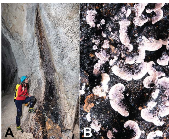
Figure 12. Actinobacterial colonies in Clearwater Cave. A) A crack in the bedrock allows organic carbon-rich water to enter the cave, which promotes microbial growth. Due to the complex chemistry of this organic carbon, microbial communities dominated by members of the Actinobacteria, which can break it down, are dominant. B) The dark patina of the rock makes the calcification of these colonies more obvious, with a radiating pattern following both the molecular flow of water and the growth of the microbial colony escaping entombment in calcite.
