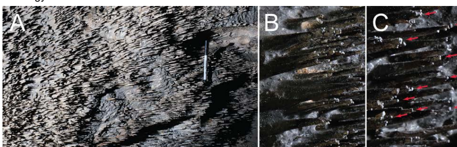
Figure 2. Phytokarst in the entrance to Clearwater Cave. A) A wall of phytokarst pinnacles pointing toward daylight (sharpie pen for scale). The area of the wall covered in this phytokarst is approximately 1.5 m high and 6 m wide. B) A close-up of individual pinnacles (the pinnacles have an average length of 3.5 cm, with tips 1 - 2 mm in diameter). C) The presence of what appears to be calcite tips on the top of each pinnacle (highlighted with red arrows) could provide a mechanism for protection on an area from photosynthetic dissolution, creating the apparent light-directed pinnacles.
