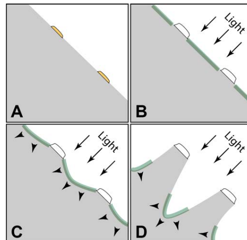
Figure 4. Model for the formation of phytokarst. Bacterial colonies are commonly found on all surfaces within the Mulu caves, and can still be seen on surfaces surrounding the phytokarst (obvious in Figure 2B). These colonies form independently of light exposure ( A ). The presence of potentially toxic Ca^{2+} ions from growth on limestone rock causes these bacterial colonies to calcify, producing a small, colony-sized piece of calcite ( B ). Calcite is opaque and prevents access of light to the surface below it, limiting growth of photosynthetic species. Cyanobacterial growth (and photosynthetic activity) can still occur on other exposed surfaces, leading to dissolution ( C ). Over time, this dissolution becomes more pronounced, and only the region originally protected by the calcite remains intact, resulting in the formation of calcite-capped pinnacles ( D ).
