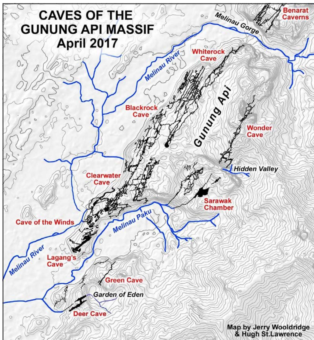
Figure 1.4: Caves of the Gunung Api Massif after the 2017 Expeditions
