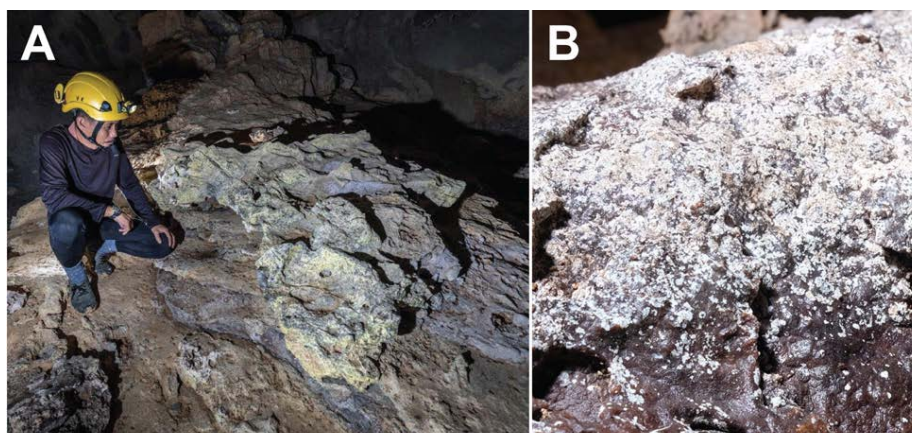
Figure 11. Microbial growth on surfaces throughout the Mulu caves. A) Microbial growth on high-moisture surfaces creates a white patina that gives many surfaces within the caves a grayish hue. B) A close up of microbial growth demonstrates how individual microbial colonies merge together to cover surfaces (Photo in A by Chris Howes).
