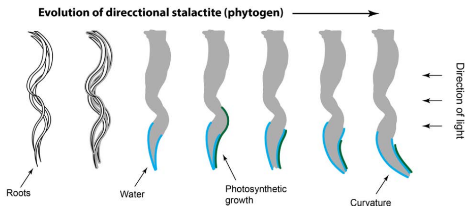
Figure 7. Formation of curved stalactites (phytogens). The initial formation of phytokarren occurs via the abiotic mechanism. \text{CO}_2 dissolved in water forms weak carbonic acid that dissolves \text{CaCO}_3 as it moves through the rock, creating a solution in equilibrium with respect to calcite. When this water reaches the atmosphere, \text{CO}_2 off-gases and the pH rises, increasing the saturation index for calcite, which starts to precipitate. The water dripping from the ceiling may take a preferential flow path, usually through a crack, which may also be exploited by plant roots. As the water emerges, it tends to follow any root present due to adhesion forces. Thus, the calcite preferentially precipitates along this path and entombs the root. Due to its location in a cave entrance, one side of the speleothem faces toward sunlight, and a significant cyanobacterial biofilm forms, which is apparent as a bright green coating (Figure 4C). As the cyanobacteria carry out photosynthesis, they consume additional \text{CO}_2 , further increasing pH and driving additional calcification. The cyanobacterial exopolysaccharides (EPS) in the biofilm create a charge surface, which coordinates the \text{Ca}^{2+} ions and further drives precipitation. The acceleration of calcite deposition leads to the formation of a soft, microcrystalline tufa, filled with both cyanobacterial cells and EPS. As cyanobacteria preferentially grow in wet conditions, there is greater calcification where the water is highest, which is the tip of the speleothem. This leads to an even more pronounced turn toward the sunlight (Figure 4B).
